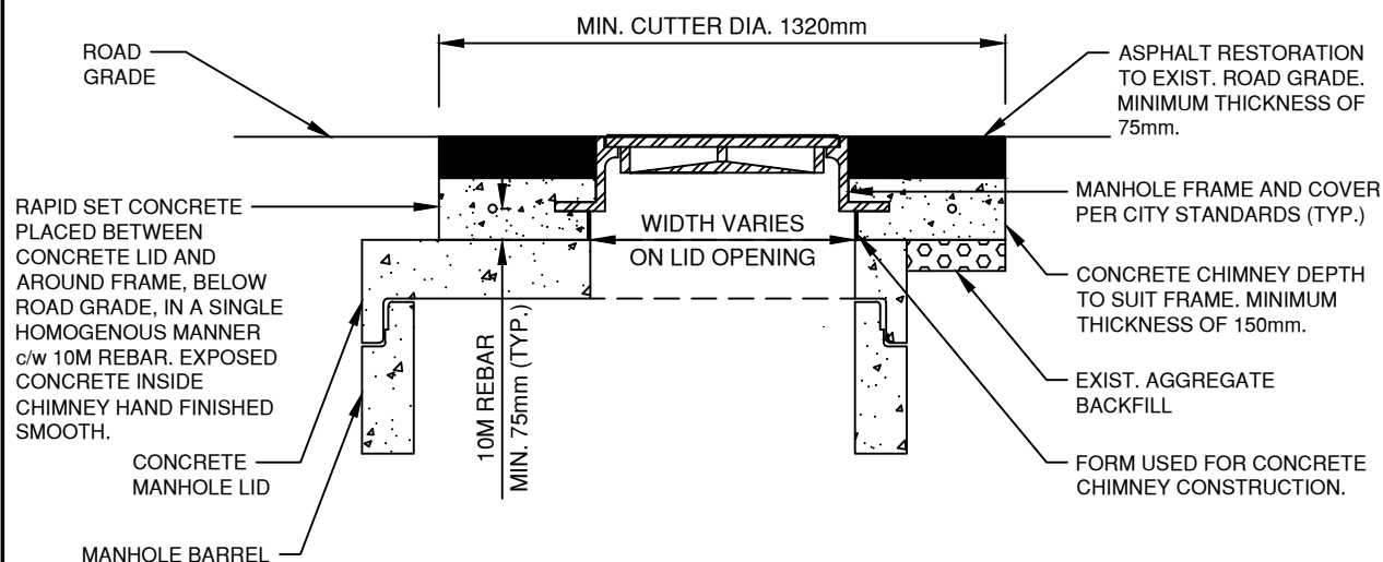
STYLE 1: RECONSTRUCTION BELOW ASPHALT GRADE
