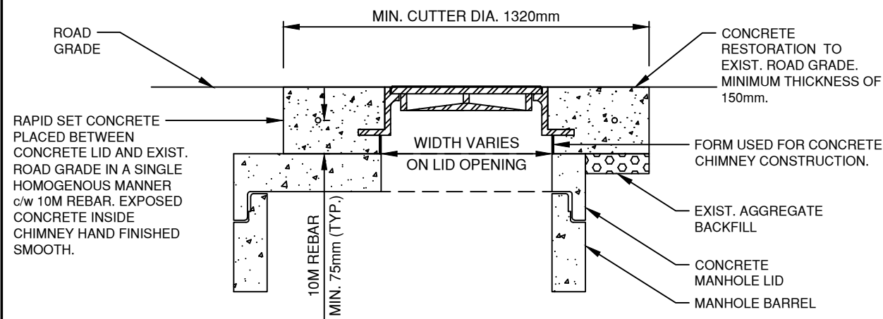
STYLE 2: RECONSTRUCTION TO FINISHED GRADE
